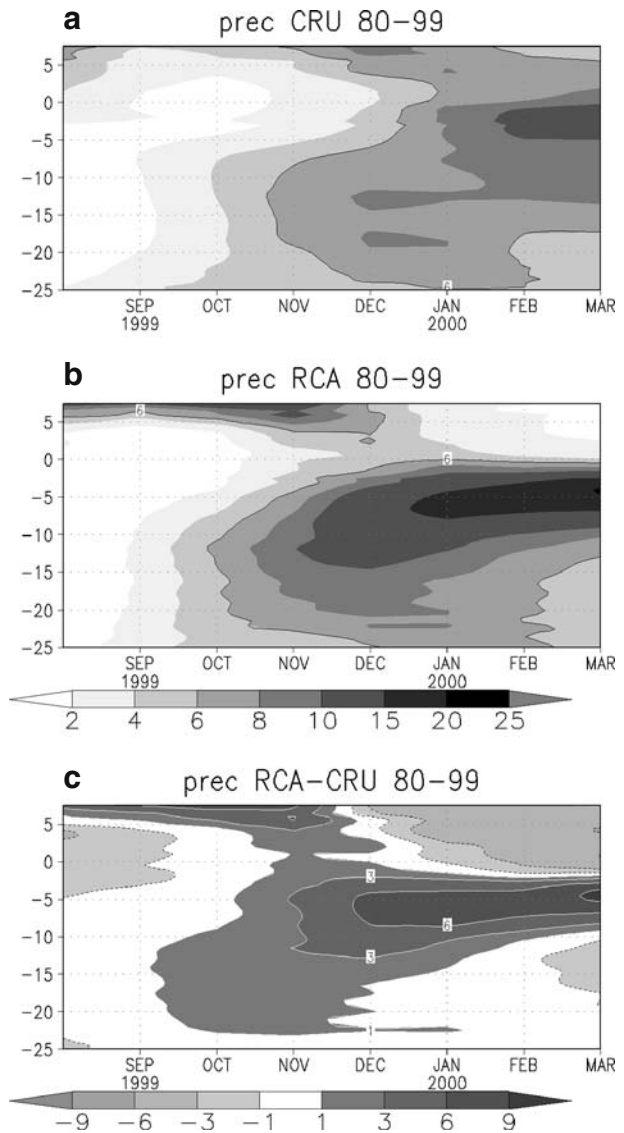
Fig. 2 Temporal evolution of the monthly mean precipitation (mm/day) averaged over 40°–60° W (land only) from August through March: a CRU, b RCA3-E, and c RCA3-E minus CRU. Vertical axis shows latitudes
