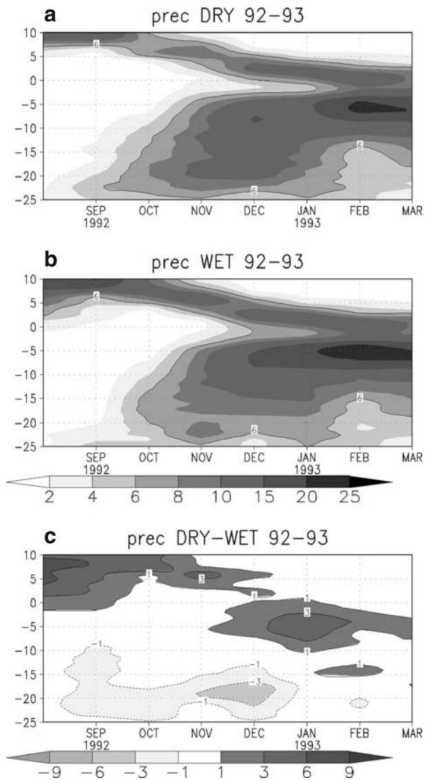
Fig. 7 Temporal evolution of the monthly mean precipitation (mm/day) averaged over 40°–60° W from August through March: a DRY, b WET, and c DRY minus WET. Vertical axis shows latitudes
